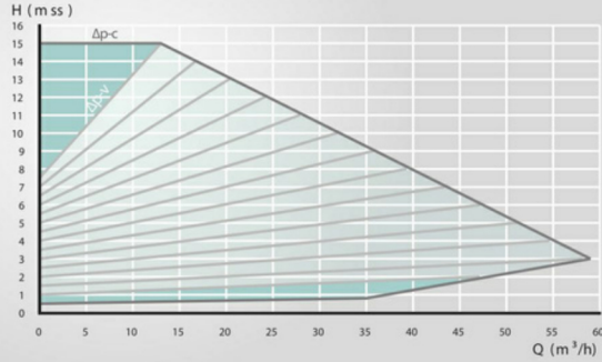
ASP 80/15 360 İNV
